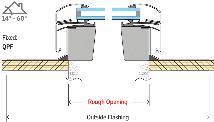
QPF - Fixed skylight
